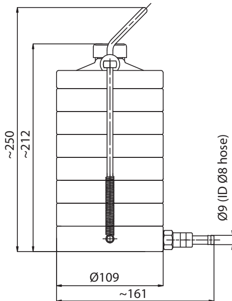
Andersen-type six stage viable cascade impactors
